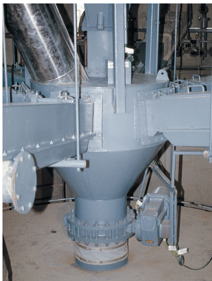
Figure 4: LOW kiln feed tank inlet
