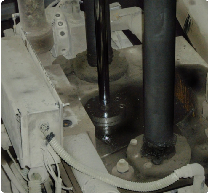
Example of a poorly maintained loading head
