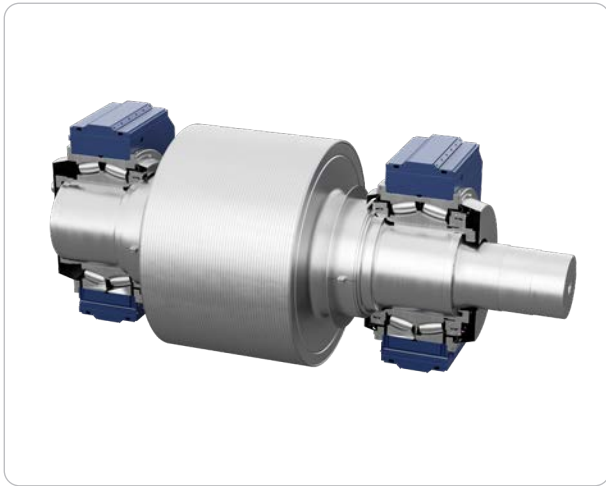
The solid forged roller shafts ensure high degree of reliability and smooth operation.
