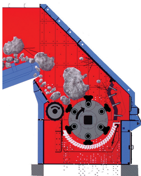
Apron feeder and one inlet roller
